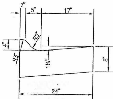
ROLLED CURB
