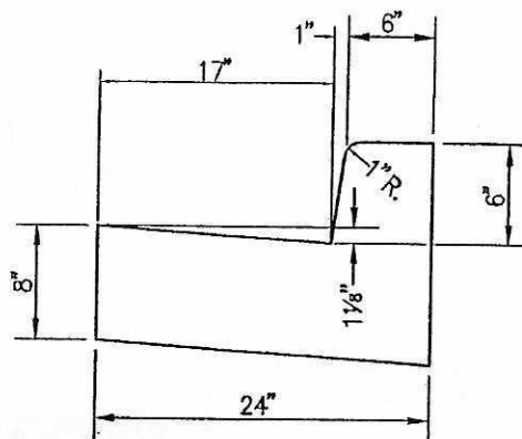
BARRIER CURB
